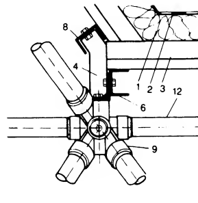
⑫ Common centre joint
